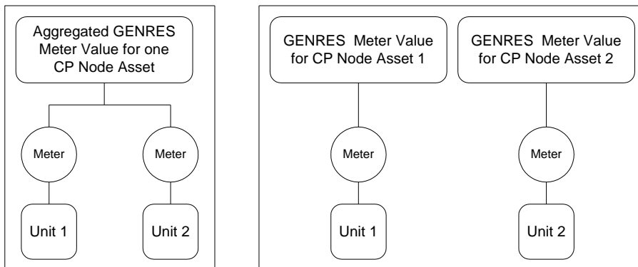
Exhibit 2-14: Combined Cycle Unit Metering
