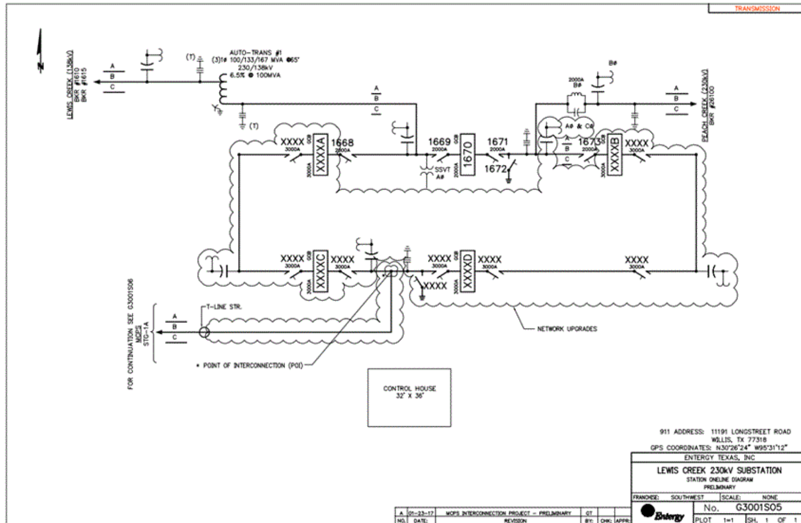
A2-2a: Transmission Owner One-Line Diagram (230kV Lewis Creek Substation)
