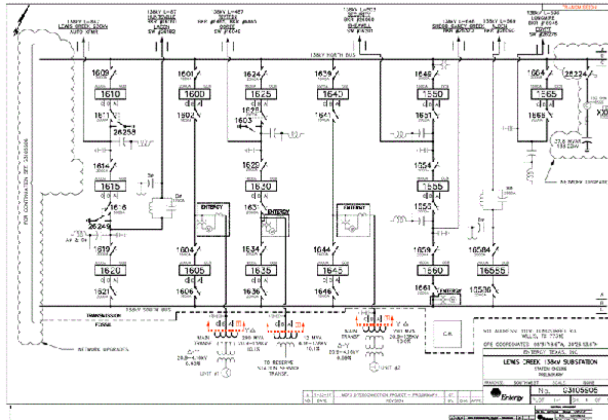
Exhibit A2. Transmission Owner One-Line A2-1a: Transmission Owner One-Line Diagram (138kV Lewis Creek Substation)
