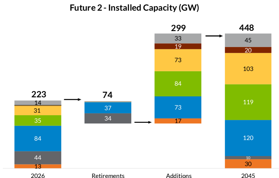
Figure 35: F2 ICAP Retirements & Additions, GW
