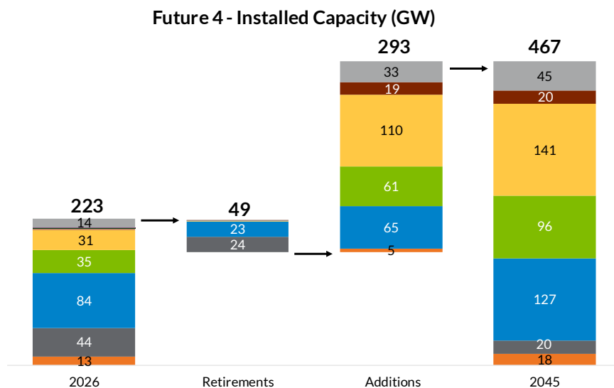
Figure 43: F4 Installed Capacity Retirements & Additions
