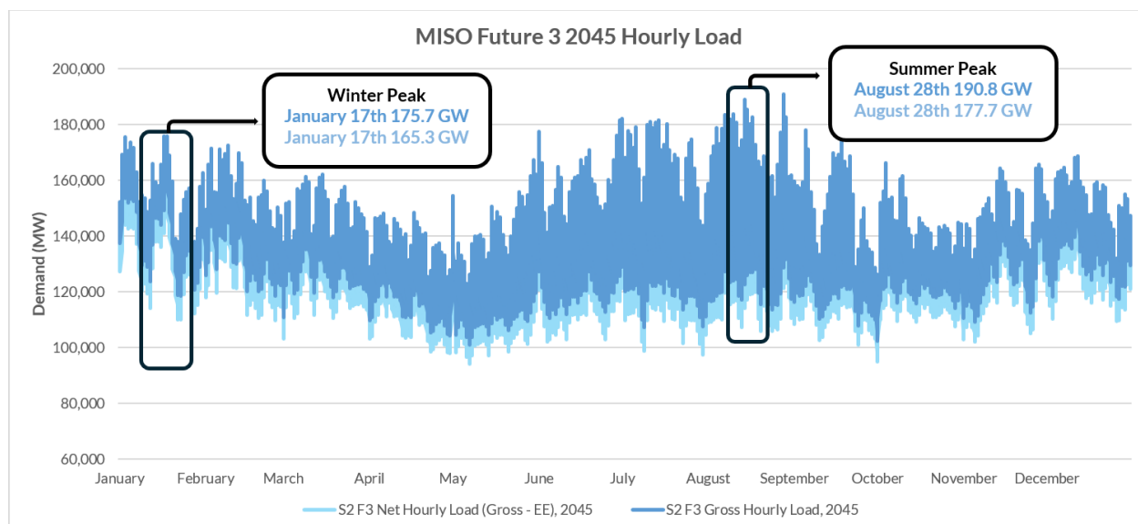
Figure 21: Hourly Net Load Shape for Series 2 Future 3, 2045
