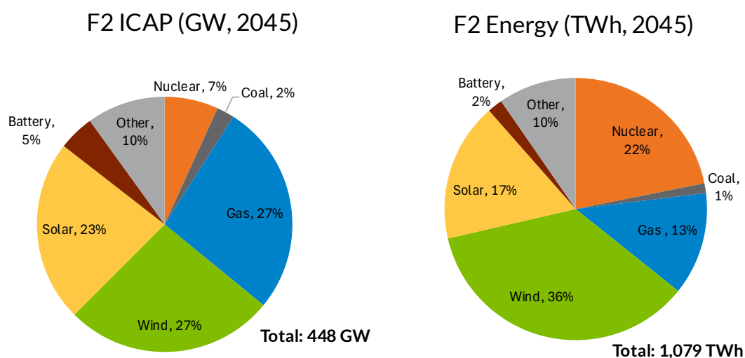
Figure 33: Future 2 Total ICAP & Energy by Resource Type, 2045
